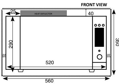
MW-1-COMBI
