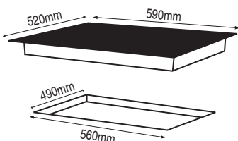
600mm Frameless Induction Hob with Touch Controls HO-4-6NF-INDUCT1
