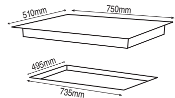
750mm Stainless Steel Low Profile 4 Gas & 1 Wok Burner Hob HO-2-75S-4GW
