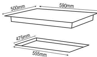
600mm Stainless Steel/White 3 Gas & 1 Wok Burner Hob HO-1-6S-3GW / HO-1-6W-3GW
