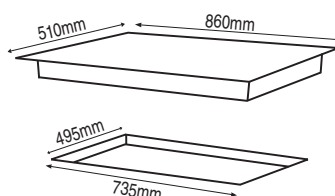
900mm Stainless Steel Low Profile 4 Gas & 1 Wok Burner Hob HO-2-9S-4GW
