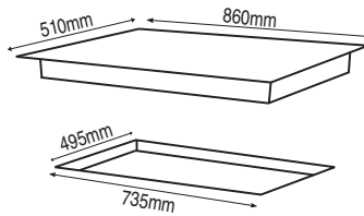
900mm Black Glass 4 Gas & 1 Wok Burner Hob HO-7-9G-4GW
