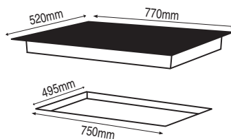
770mm Frameless Ceramic Hob with Touch Controls HO-4-77NF-CER-T
