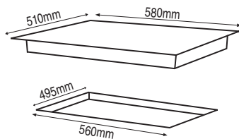
600mm Stainless Steel Low Profile 4 Gas Burner Hob HO-2-6S-4G
