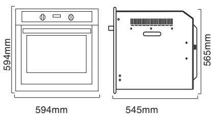
8 Function Electric Inbuilt Oven (8 Series) OV-1-6W-8 / OV-1-6S-8, OV-2-6S-8, OV-4-6W-8 / OV-4-6S-8
