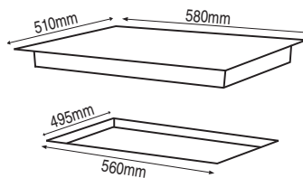
600mm Stainless Steel 3 Gas & 1 Wok Burner Hob HO-6-6S-3GW
