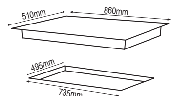
900mm Stainless Steel 4 Gas & 1 Wok Burner Hob HO-6-9S-4GW
