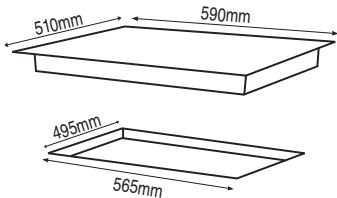
600mm Black Glass 3 Gas & 1 Wok Burner Hob HO-7-6G-3GW
