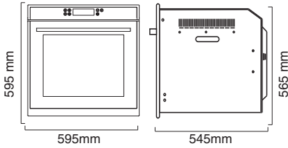
8 Function Electric Touch Inbuilt Oven PPOV-6S-70
