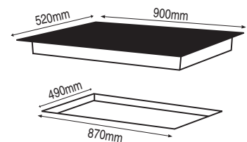
900mm Frameless Ceramic Hob with Touch Controls HO-4-9NF-CER-T-1
