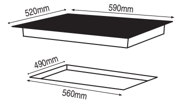
600mm Frameless Ceramic Hob HO-4-6NF-CER
