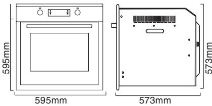
10 Function Electric Pyrolytic Inbuilt Oven PPOV-6S-PYRO-1
