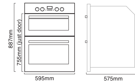
8+2 Function Electric Double Inbuilt Oven PPOV-6S-DT-1
