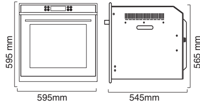
9 Function Electric Multi-zone Inbuilt Oven PPOV-6S-MULTI
