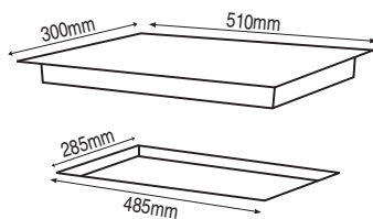
300mm Stainless Steel 2 Gas Burner Domino Hob HO-1-2S-2G
