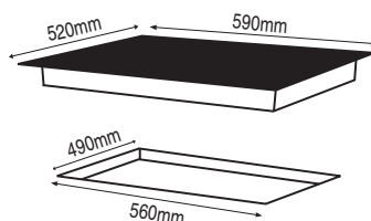
600mm Zoneless, Frameless Induction Hob with Touch Controls HO-4-6NF-ZLINDUCT
