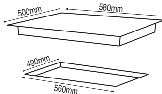
600mm White & Stainless Steel 4 Element Electric Hob HOB6S-4E-4 / HOB6W-4E-4
