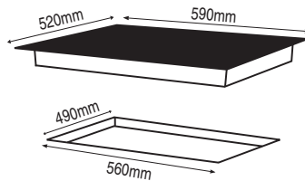
600mm Ceramic Hob, Stainless Steel frame HO-4-6S-CER / HO-4-6S-CER-T
