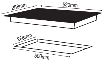
Ceramic Domino Hob with Touch Controls HO-4-2NF-CER-T
