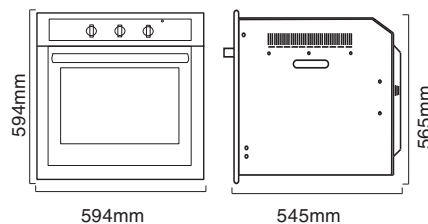
5 Function Electric Inbuilt Oven (5 Series) OV-1-6W-5 / OV-1-6S-5, OV-2-6S-5, OV-4-6S-5
