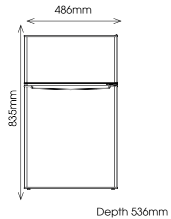
Underbench 88L Fridge Freezer FR-88W-UBF
