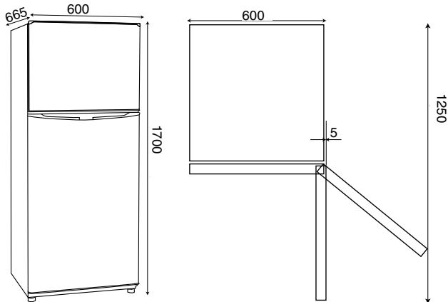
Single Door 366L Fridge Freezer FR-366STM-FF
