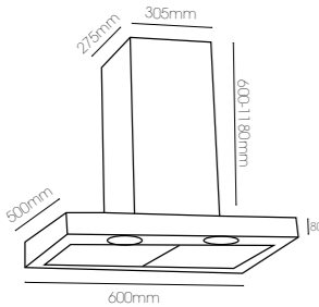
600mm Stainless Steel Box Canopy RBOX-6S-1000L
