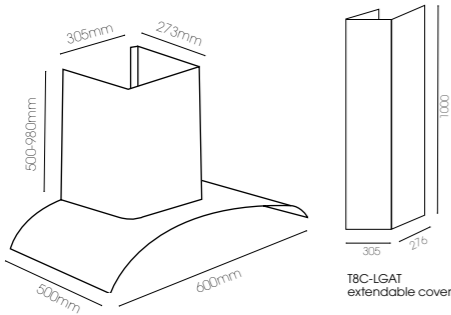
600mm Curved Glass Canopy T4-11GLA-6L
