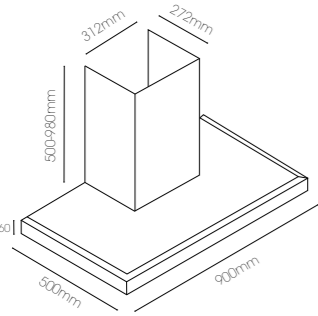
900mm Stainless Steel Peripheral Box Canopy RPER-9G-1000
