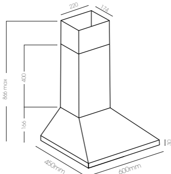
600mm Stainless Steel Pyramid Canopy RC6W550
