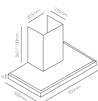
900mm Stainless Steel Digimax LCD Box Canopy RLCD-9G-1000L
