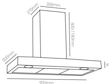
900mm Stainless Steel Box Canopy RBOX-9S-1000L
