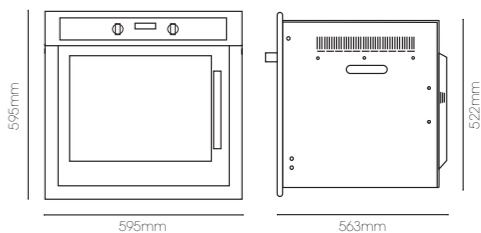
7 Function Electric Side Door Oven PPOV-6S-SIDE-1
