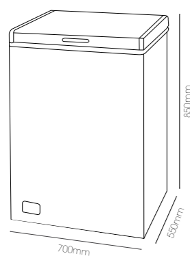
145L Chest Freezer CHF-145
