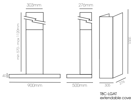
900mm Stainless Steel Slimline Box Canopy T4-12LOW-9L
