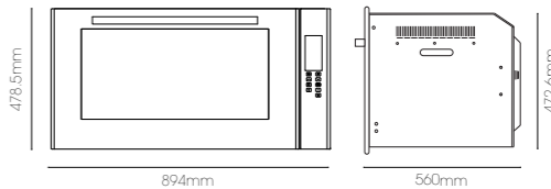
10 Function, 900mm Electric Touch Inbuilt Oven PPOV-9S-48
