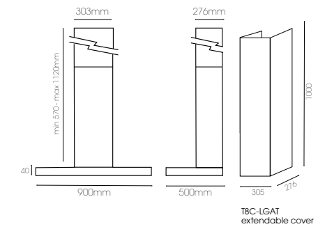
900mm Stainless Steel Slimline Box Canopy T4-12LOW-9L
