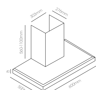
600mm Stainless Steel Digimax LCD Box Canopy RLCD-6G-1000L
