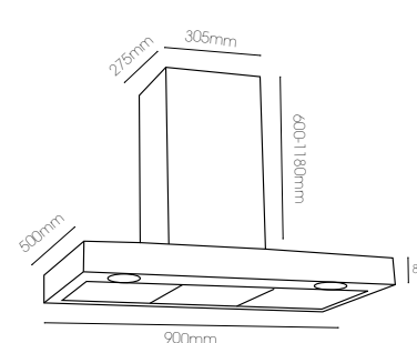
900mm Stainless Steel Box Canopy RBOX-9S-1000L
