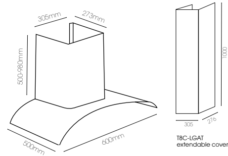
600mm Curved Glass Canopy T4-11GLA-6L
