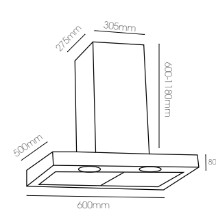
600mm Stainless Steel Box Canopy RBOX-6S-1000L
