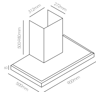
900mm Stainless Steel Peripheral Box Canopy RPER-9G-1000
