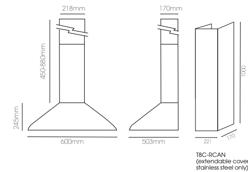
600mm Stainless Steel Pyramid Canopy RC6W550
