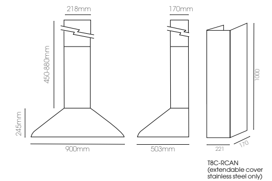
900mm Stainless Steel / White / Black Pyramid Canopy (500 & 1000) RCAN-9S-500L / RCAN-9W-1000L RCAN-9S-1000L / URCAN-9B-1000L
