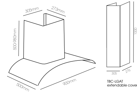
900mm Curved Glass Canopy T4-11GLA-9L
