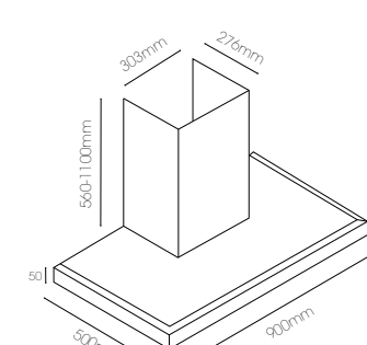
900mm Stainless Steel Digimax LCD Box Canopy RLCD-9G-1000L
