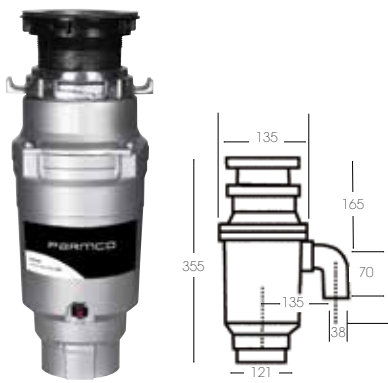
STANDARD WASTE DISPOSAL GD-2
