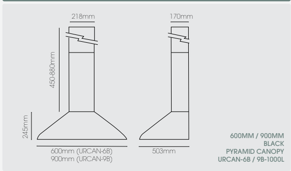
UNBRANDED LIFESTYLE 1000 CANOPY URCAN-6B / 9B-1000L
