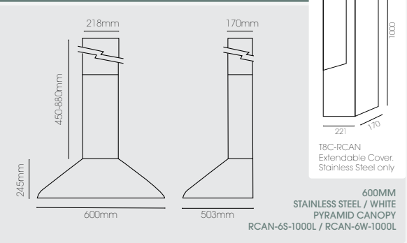
LIFESTYLE 1000 CANOPY RCAN-6S-1000L / RCAN-6W-1000L
